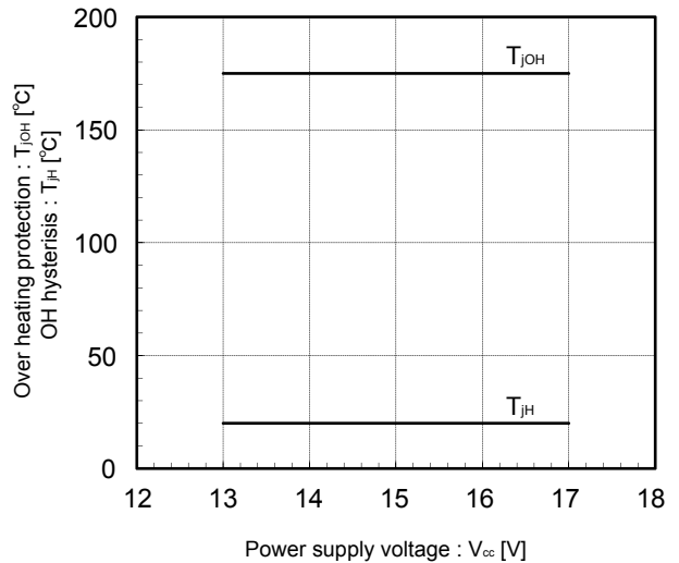
Over heating characteristics T_{OH}, T_{jH} vs. V_{cc} (typ.)
