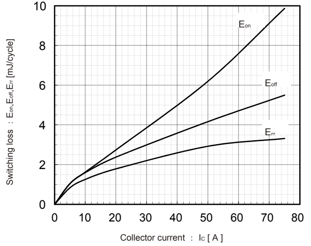
Switching Loss vs. Collector Current (typ.) V_{DC}=600V, V_{CC}=15V, T_J=125^\circ C
