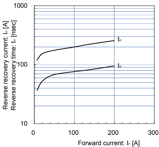
Reverse Recovery Characteristics (typ.) V_{CC}=300V, V_{GE}=\pm 15V, R_G=13\Omega, T_J=150^\circ C
