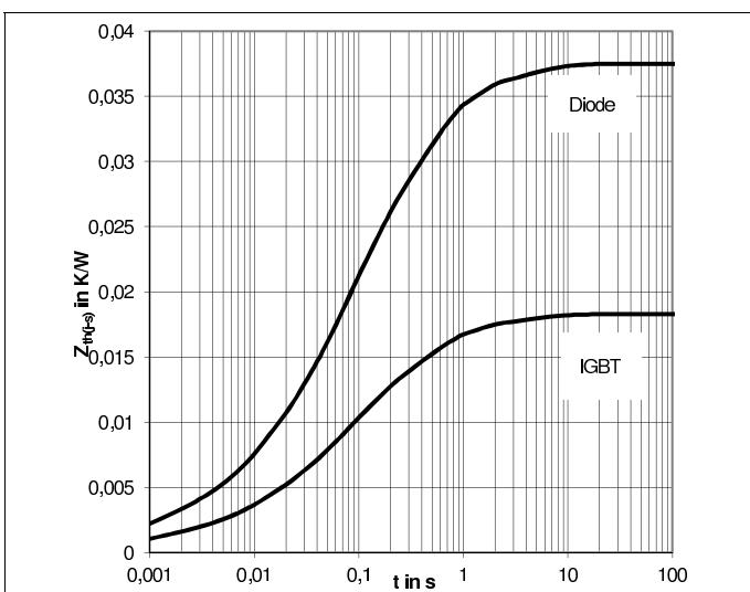
Fig. 5: Transient thermal impedance Z_{th}(j-r)
